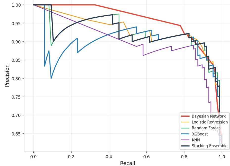
Precision-Recall Curves — All Models
