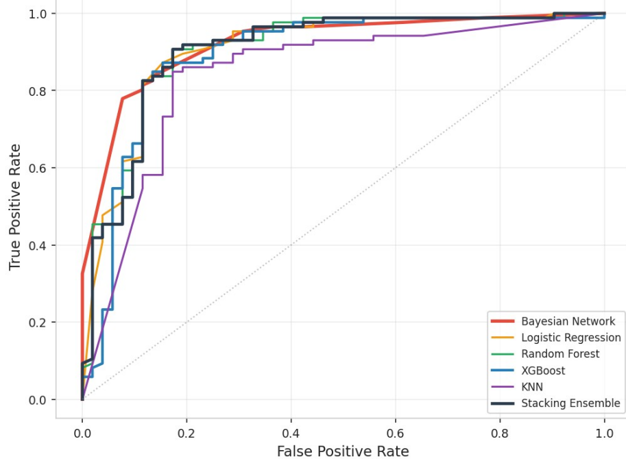
ROC Curves — All Models
