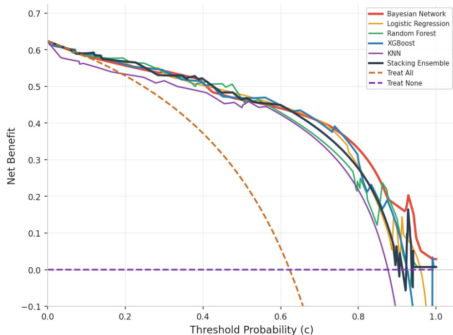
Decision Curve Analysis — All Models
